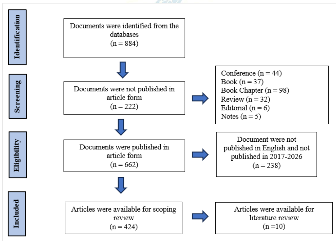
Figure 1. PRISMA flowchart
